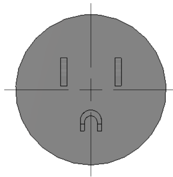
Hospital Grade Plug NEMA 5-15P molded on 2 foot power cord For 15A 120V
