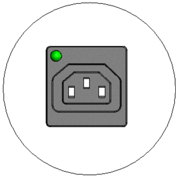
IEC 60320 C-13 Connector For 15A 250V / 10 A 250V Green LED indicates power on
